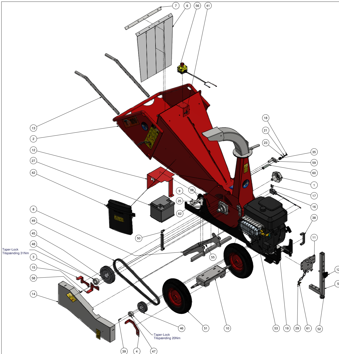
Rotor komplet TP100 MOBILE Spare parts list
