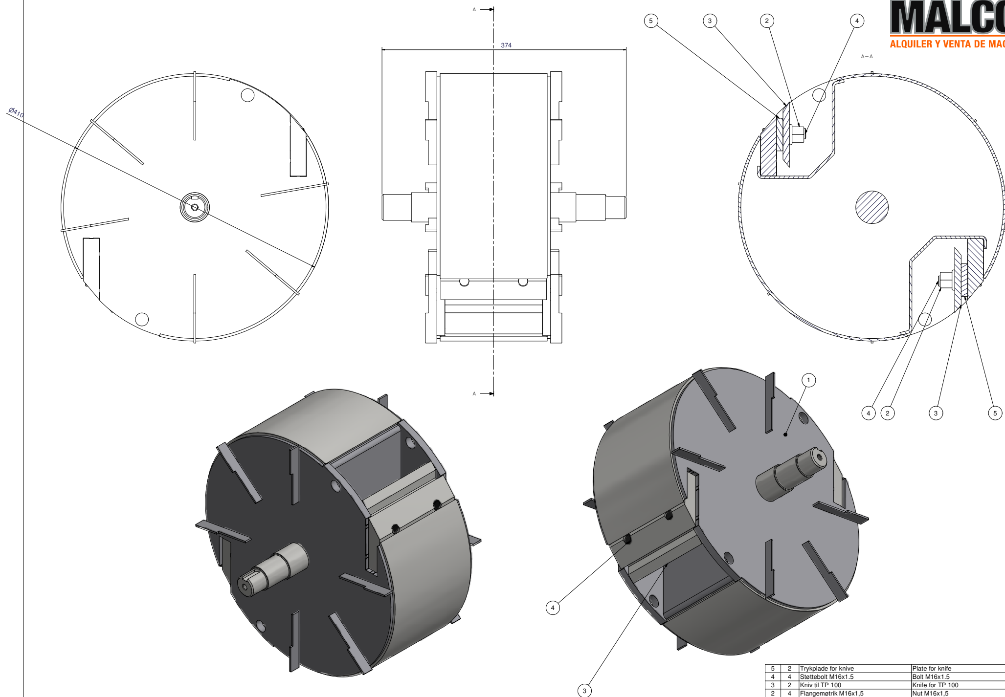
Rotor komplet TP100 MOBILE Spare parts list
